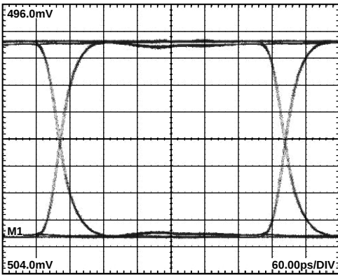
Figure 13. ADCMP572 Eye Diagram at 2.5 Gbps
