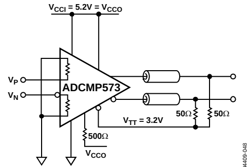
Figure 27. Disabling the ADCMP573 Latch Feature
