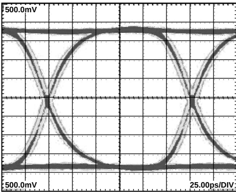
Figure 14. ADCMP572 Eye Diagram at 6.5 Gbps
