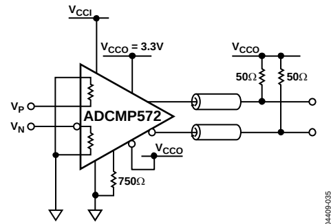
Figure 26. Disabling the ADCMP572 Latch Feature
