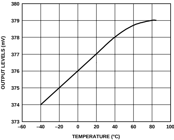
Figure 12. Output Levels vs. Temperature
