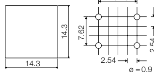
PCB layout
