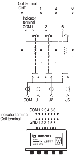
Fail-safe type
