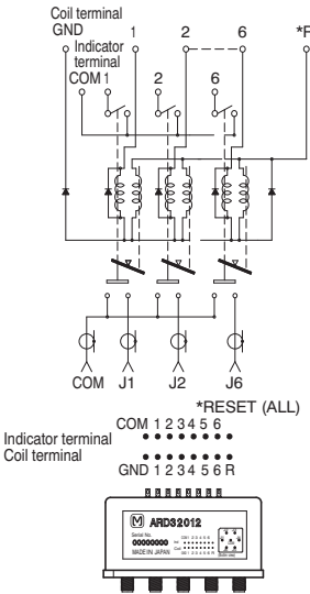
Latching type
