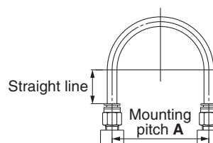
Fig. 1 Recommended piping
