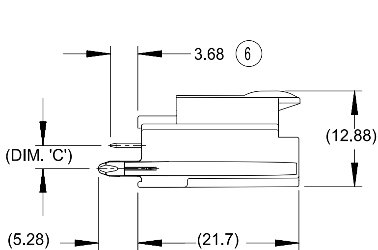
6 WAY VERTICAL HEADER ASSEMBLY (POLARIZATION OPTIONS) VIEWED FROM MATE SIDE
