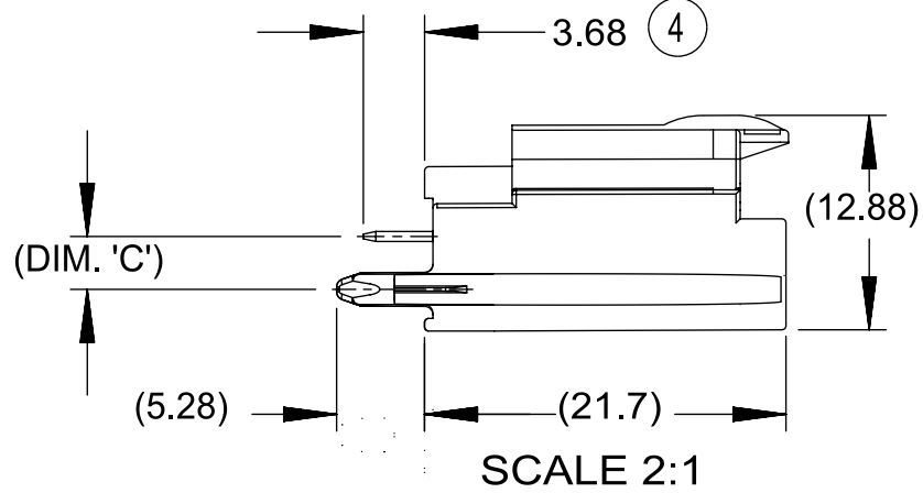
4 WAY VERTICAL HEADER ASSEMBLY (POLARIZATION OPTIONS) VIEWED FROM MATE SIDE
