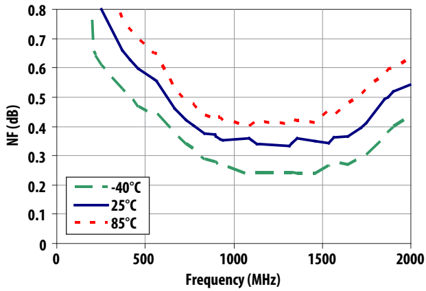
Figure 22. NF vs Frequency vs Temperature
