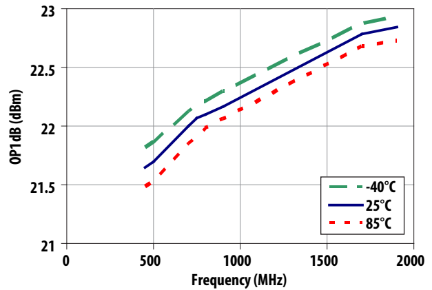
Figure 25. OP1dB vs Frequency vs Temperature
