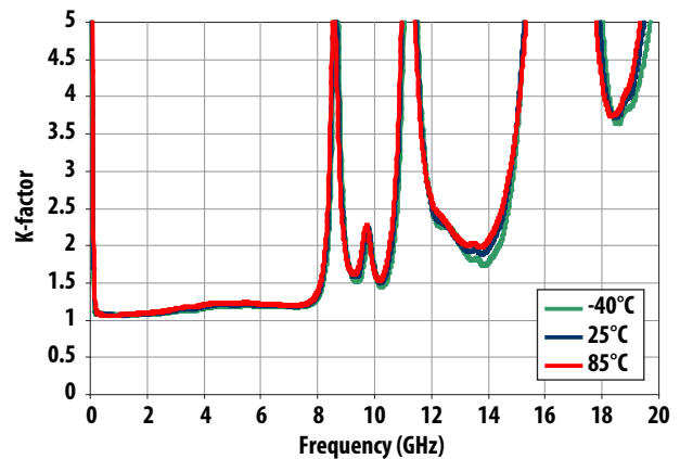
Figure 27. K-factor vs Frequency vs Temperature
