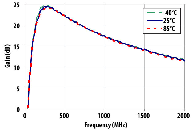
Figure 23. Gain vs Frequency vs Temperature
