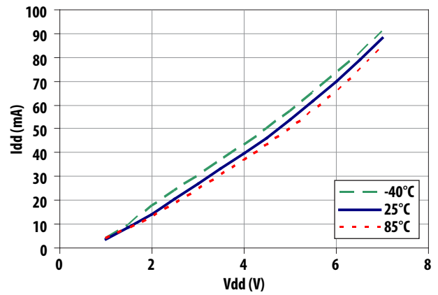
Figure 29. Idd vs Vdd vs Temperature
