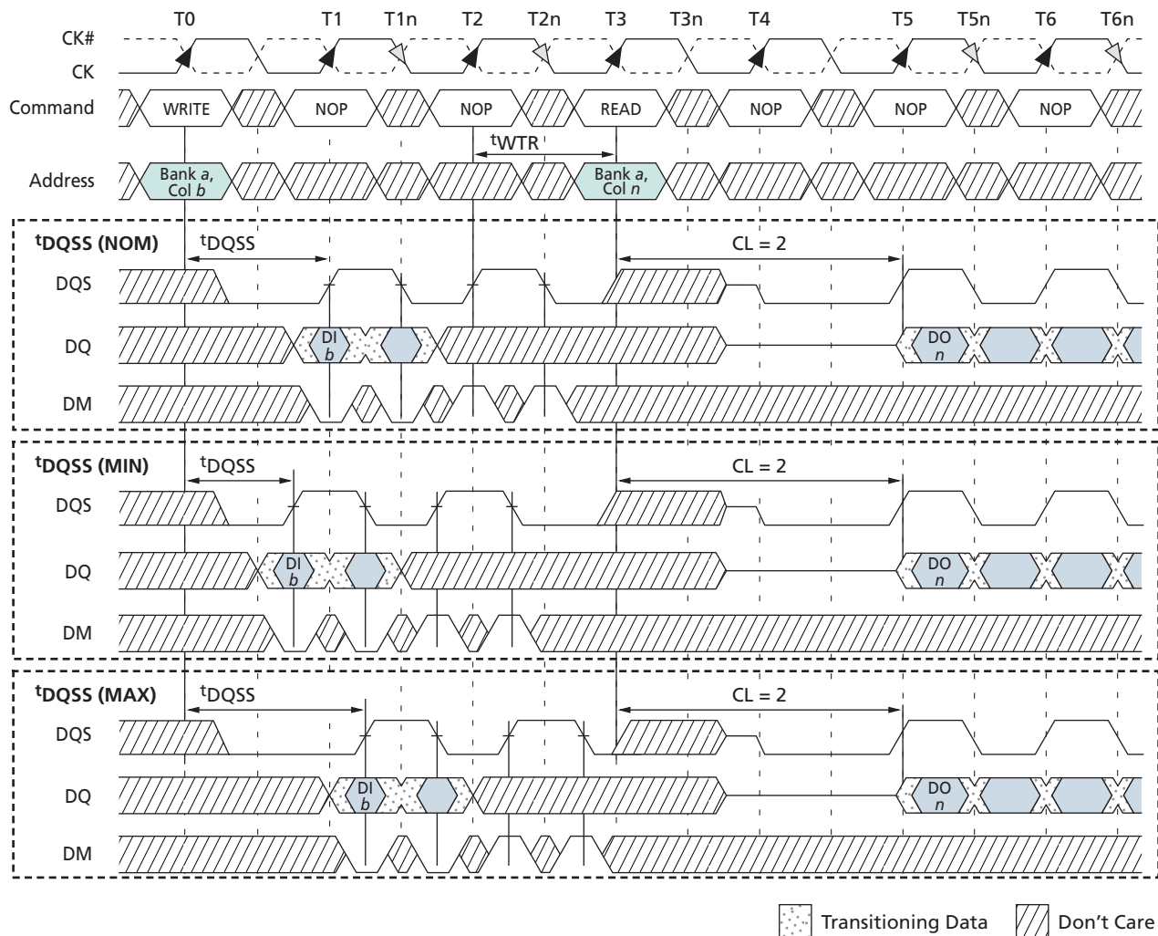
Figure 44: WRITE-to-READ – Interrupting
