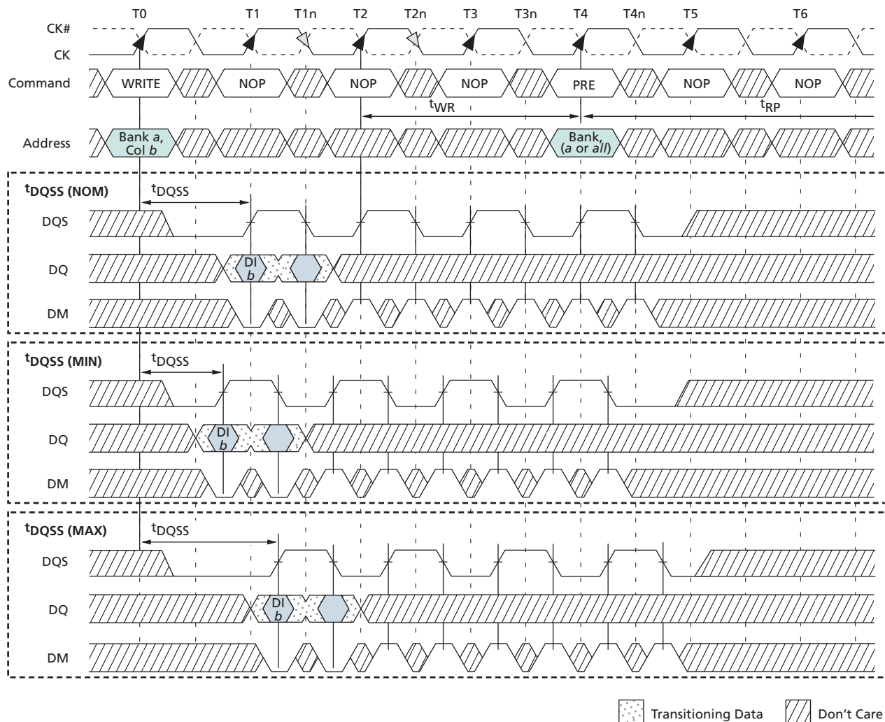
Figure 47: WRITE-to-PRECHARGE – Interrupting
