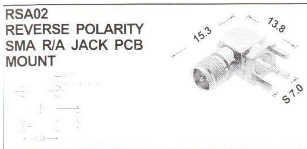
Figure 1: Right Angle Jack PCB Mount
