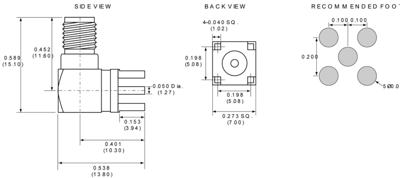
Figure 2: CON-RPSMA-RA Dimension Specifications
