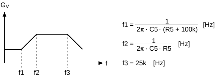
Figure 3 Frequency Characteristic of MS AMP
