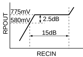
Figure 5 ALC Operation Level
