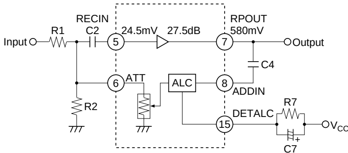
Figure 6 ALC Block Diagram
