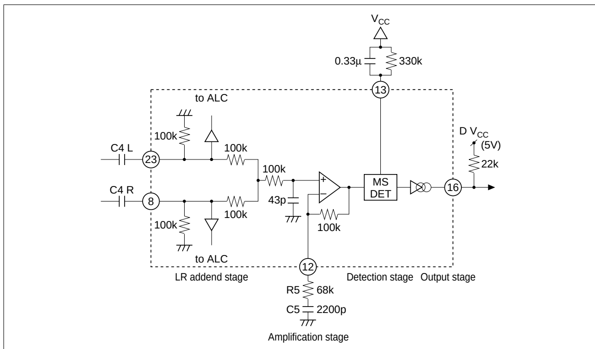
Figure 2 Music Sensor Block Diagram
