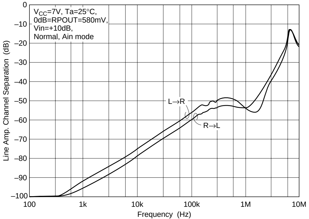
Line Amp. Channel Separation vs. Frequency
