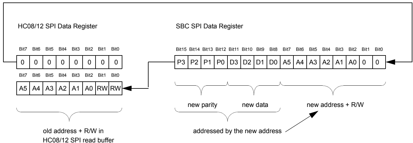
Figure 20. Microcontroller SPI Reading Data - Sequence B
