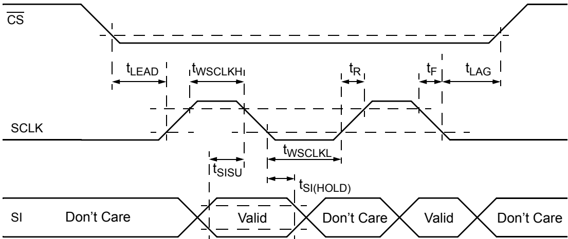
Figure 4. Input Timing Switch Characteristics
