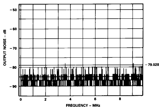
Figure 19. Noise Spectrum
