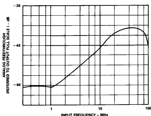
Figure 20. Analog Feedthrough vs. Frequency
