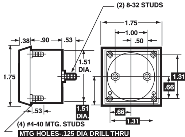
1-1/2"-Models 2121, 2121T, 2141,
