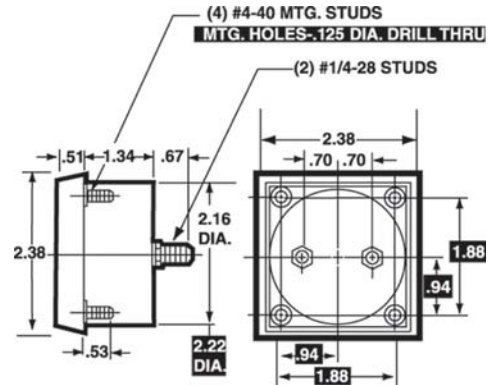
2-1/2"-Models 2122, 2122T, 2142, 2152, 2182
