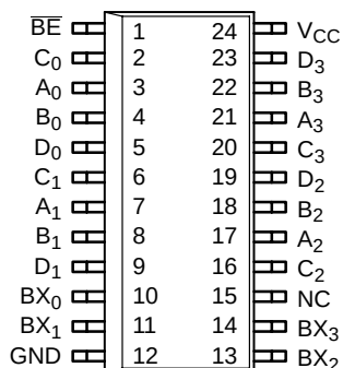
Figure 1. 24-Lead Pinout
