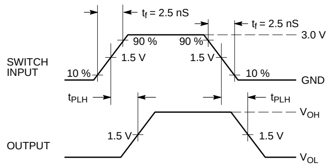
Figure 4. Propagation Delays
