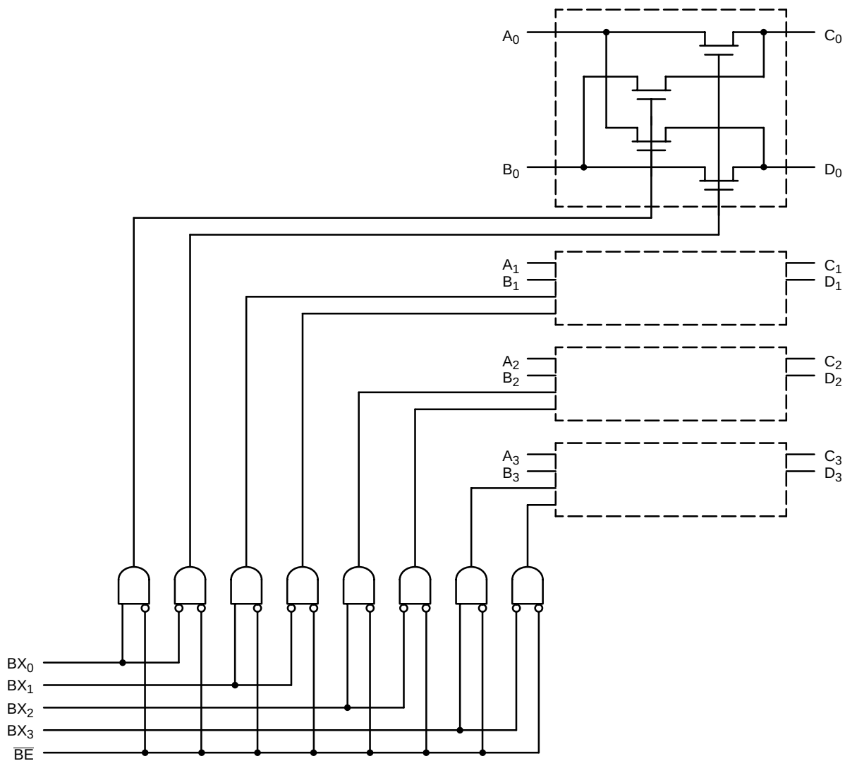
Figure 2. Logic Diagram
