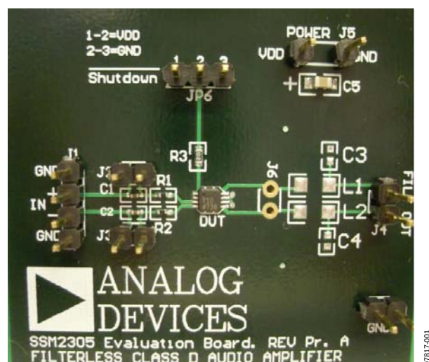
Figure 1. SSM2305 Evaluation Board, Top View
