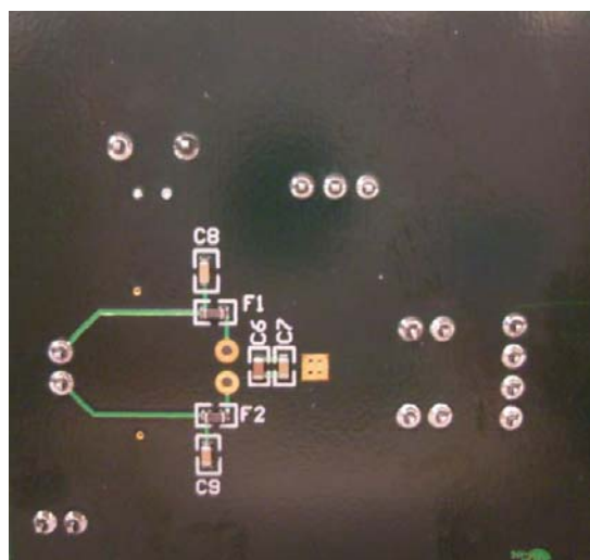
Figure 2. SSM2305 Evaluation Board, Bottom View
