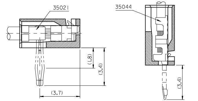
RIGHT ANGLE TYPE
