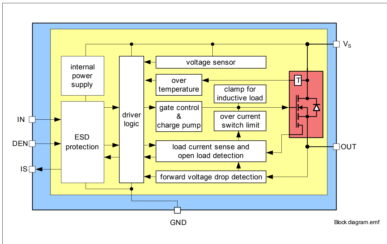
Figure 1 Block Diagram for the BTT6010-1EKB
