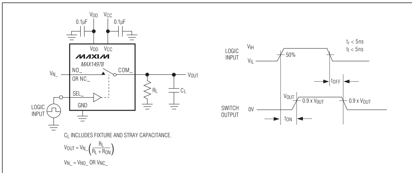
Figure 2. Switching Time
