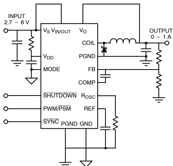
Buck Configuration
