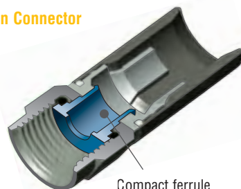
Compact ferrule
