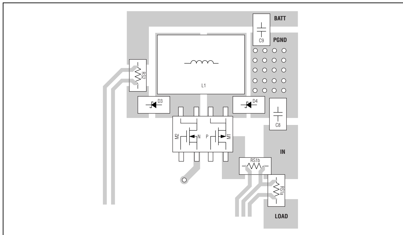
Figure 14. Recommended Layout for the MAX1870A
