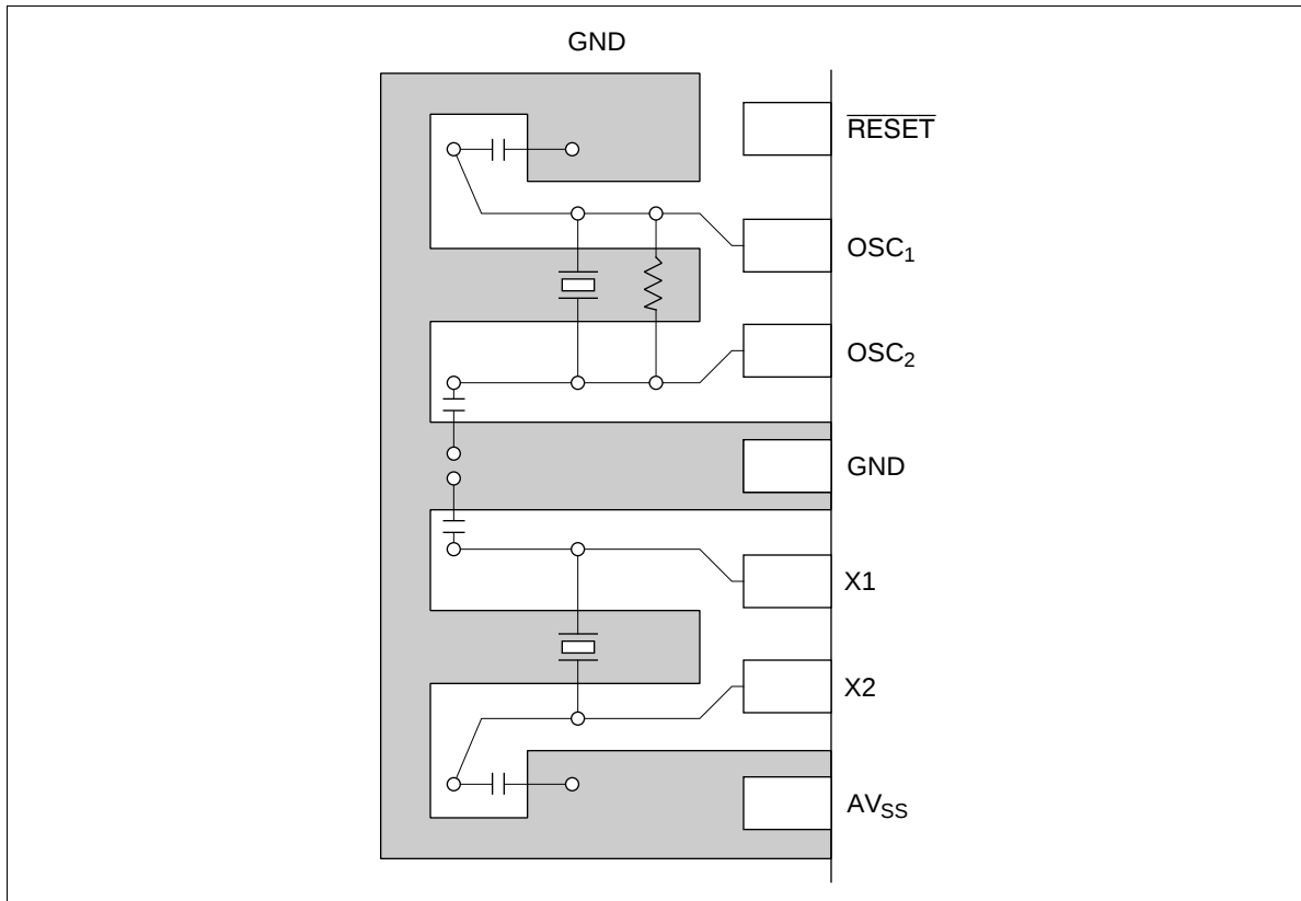
Figure 19 Typical Layout of Crystal and Ceramic Oscillators
