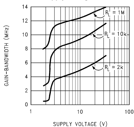
GBW vs. Supply Voltage at 20 kHz
