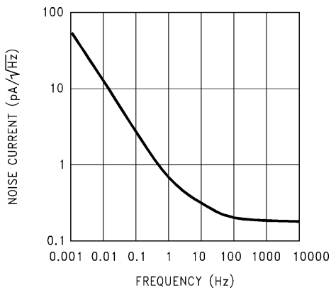
Noise Current vs. Frequency
