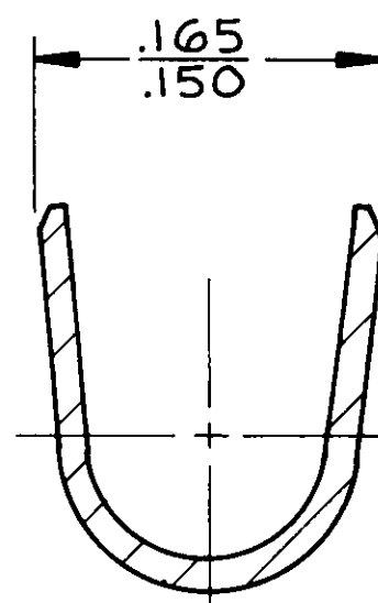
SECTION B-B
