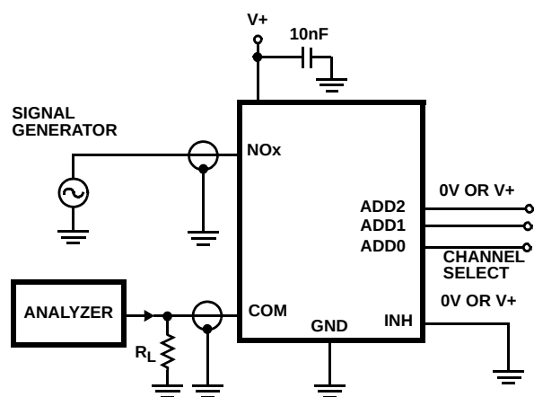
FIGURE 3. BREAK-BEFORE-MAKE TIME
