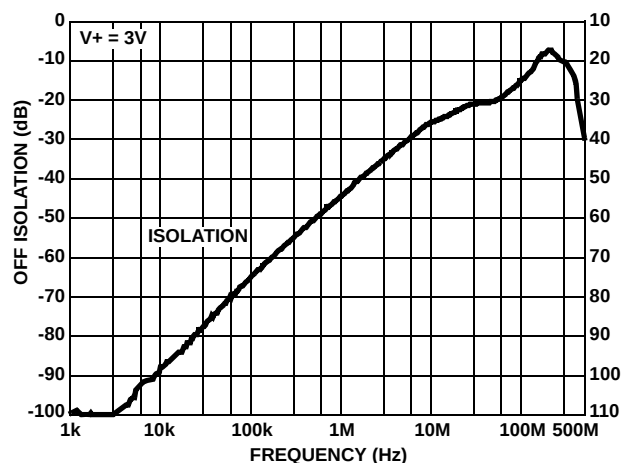
FIGURE 17. OFF-ISOLATION
