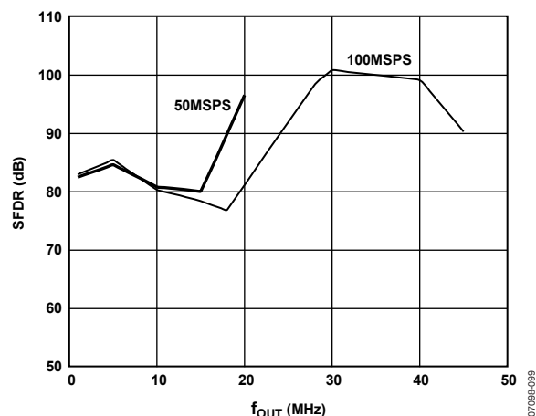
Figure 39. AD9788 In-Band SFDR vs. f_{OUT} , 8 \times Interpolation
