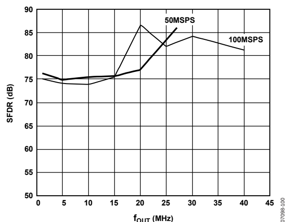
Figure 40. AD9788 Out-of-Band SFDR vs. f_{OUT} , 8 \times Interpolation
