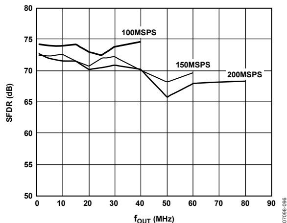
Figure 36. AD9788 Out-of-Band SFDR vs. f_{OUT} , 4 \times Interpolation
