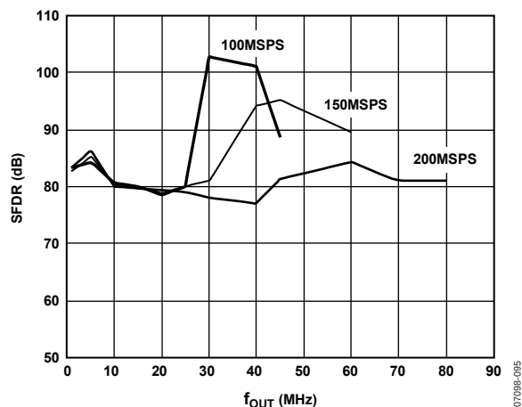
Figure 35. AD9788 In-Band SFDR vs. f_{OUT} , 4 \times Interpolation
