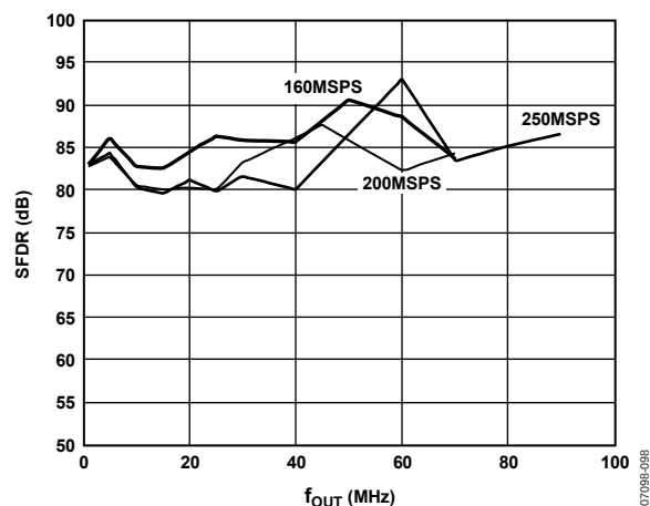
Figure 38. AD9788 In-Band SFDR vs. f_{OUT} , 2 \times Interpolation
