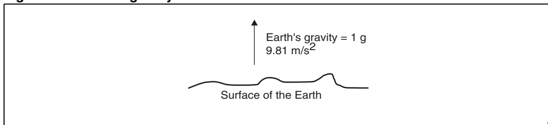
Figure 21. Earth's gravity
