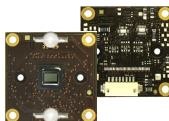
phyCAM-S (VM-007-LVDS-LED)
