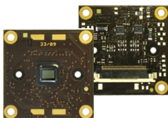
phyCAM-P (VM-007-MUX)
