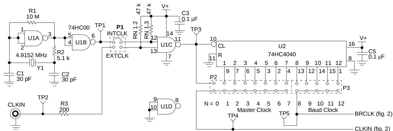
Figure 1. Clock Generator
