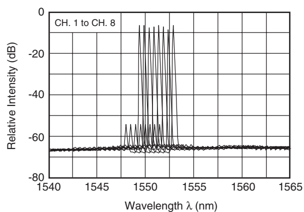
Fig. 5 Filter Curve
