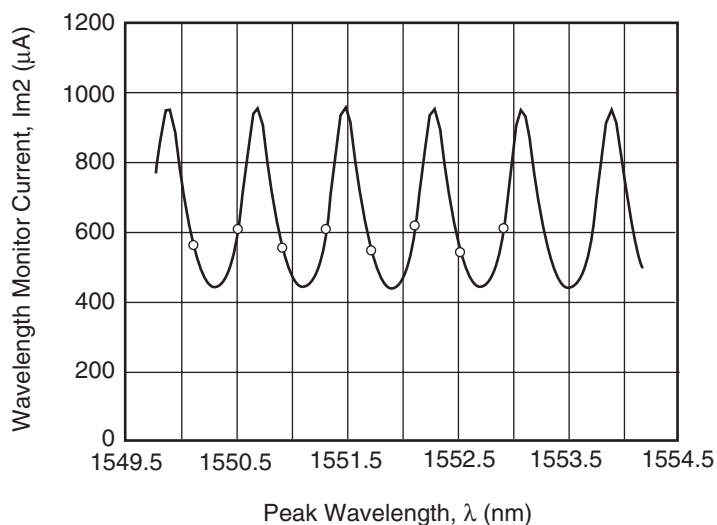
Fig. 5 Filter Curve
