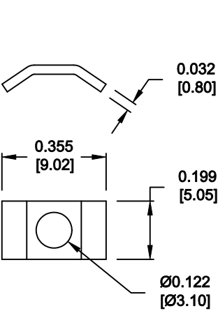
SADDLE WASHER
