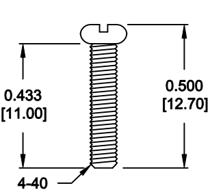
HOUSING SCREW
