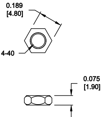
HOUSING NUT
