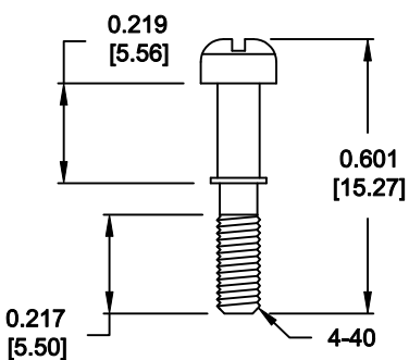
MATING SCREW
