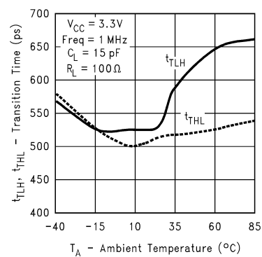
Transition Time vs Ambient Temperature
