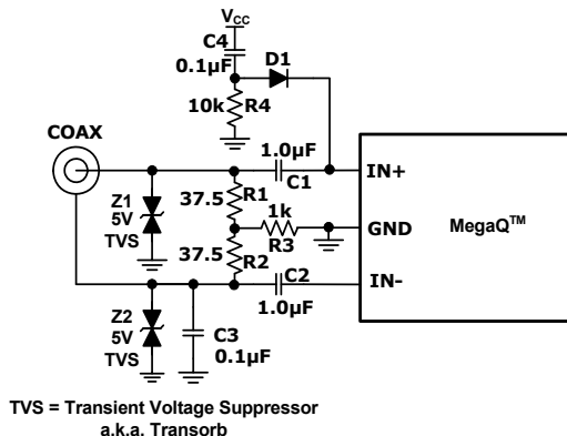
FIGURE 46. APPLICATION CIRCUIT FOR COAX CABLE
