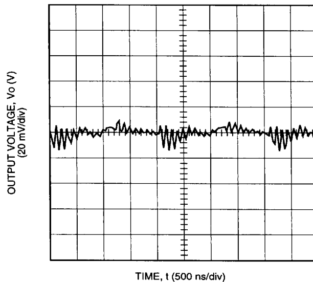
Figure 3. Typical FE200A9 Output Ripple Voltage at Room Temperature, 48 V Input, and 40 A Output
