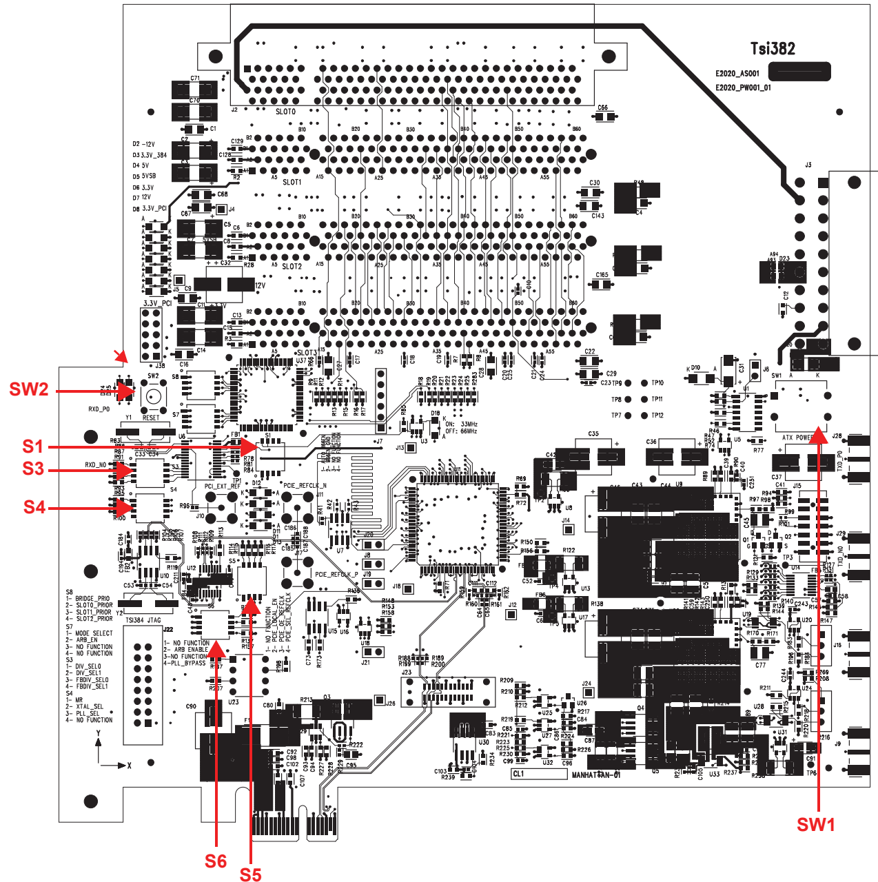
Figure 6: Switch Locations
