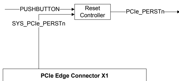
Figure 4: Board Reset
