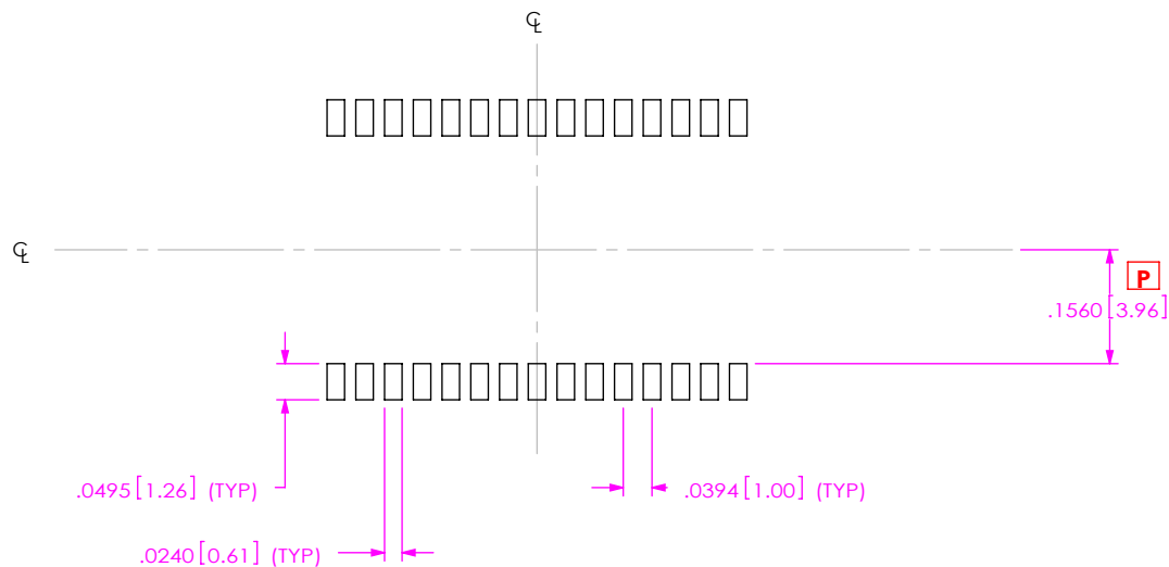
FIG 4 FOR -10, -20, -30 POSITION (THREADED) OR -05 THROUGH -50 (NON-THREADED) ALL DIMENSIONS ARE SYMMETRIC ABOUT THE CENTERLINE.
