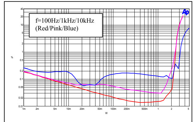
THD+N Vs. Output Power ( R_L=4\Omega )
