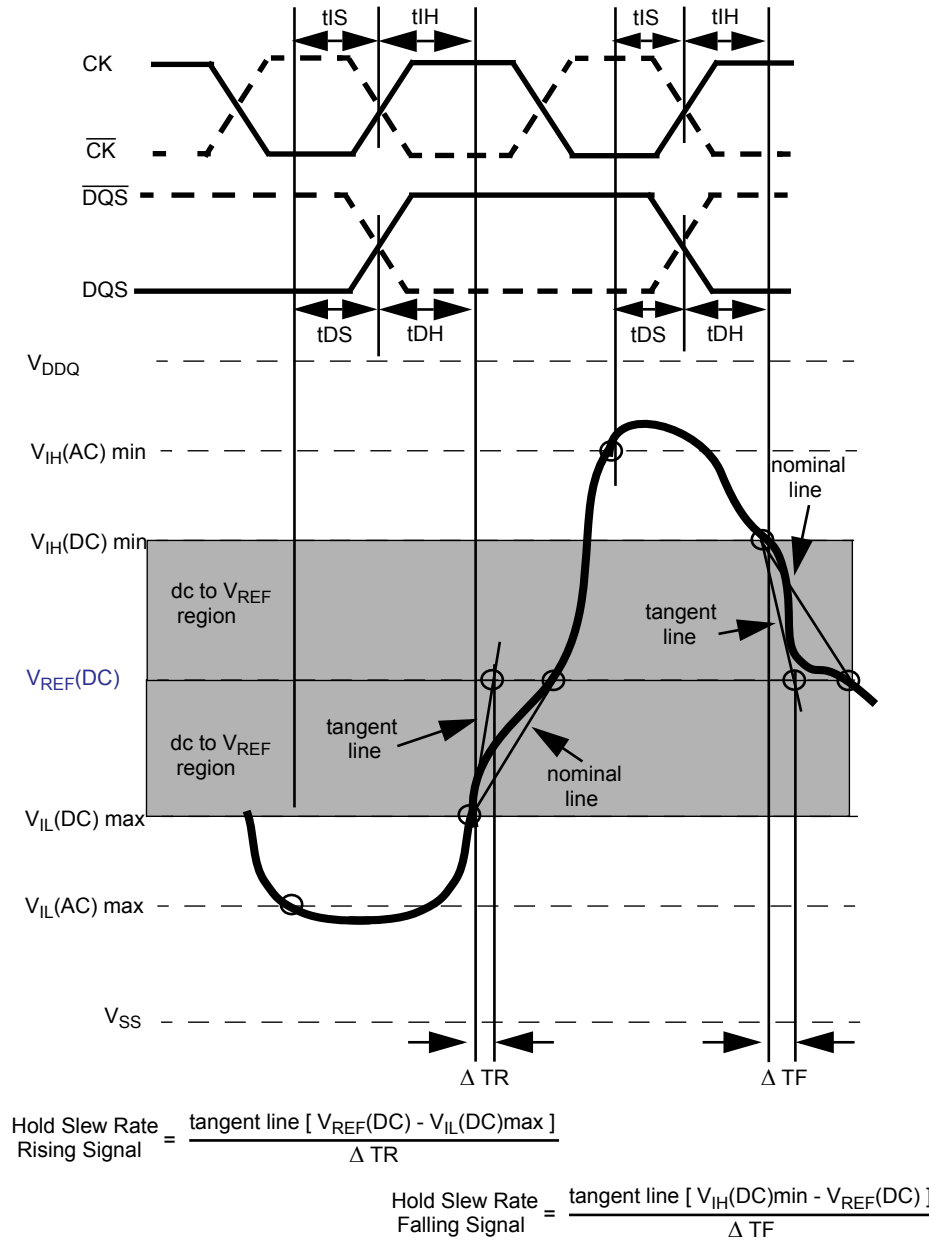
Figure 23. Illustration of tangent line for hold time t_{DH} (for DQ with respect to strobe) and t_{IH} (for ADD/CMD with respect to clock)
