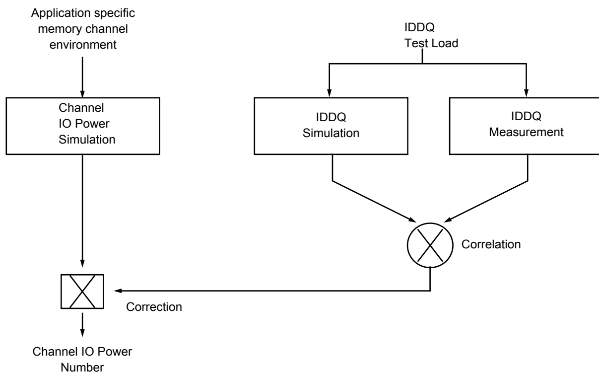
Figure 19. Correlation from simulated Channel IO Power to actual Channel IO Power supported by IDDQ Measurement.
