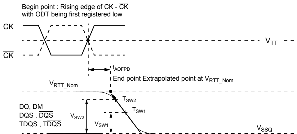
Figure 16. Definition of t_{\text{AOFPD}}
