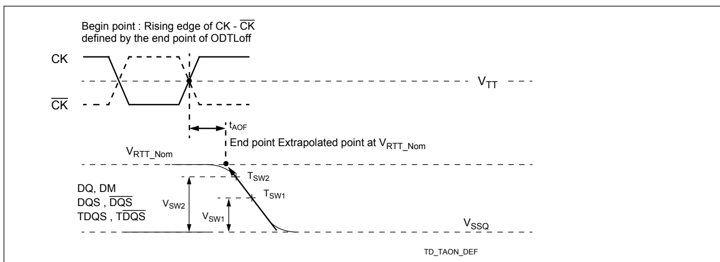
Figure 15. Definition of tAOF
