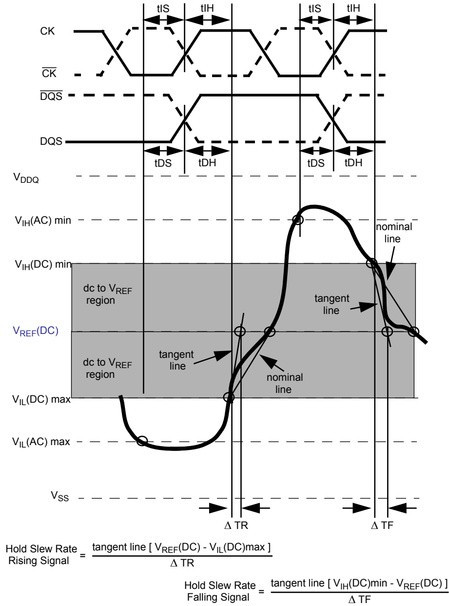
Figure 27. Illustration of tangent line for hold time t_{DH} (for DQ with respect to strobe) and t_{IH} (for ADD/CMD with respect to clock)
