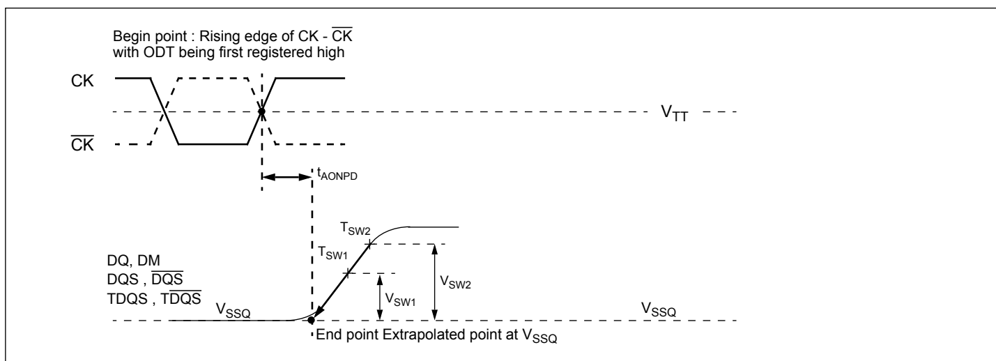
Figure 14. Definition of tAONPD
