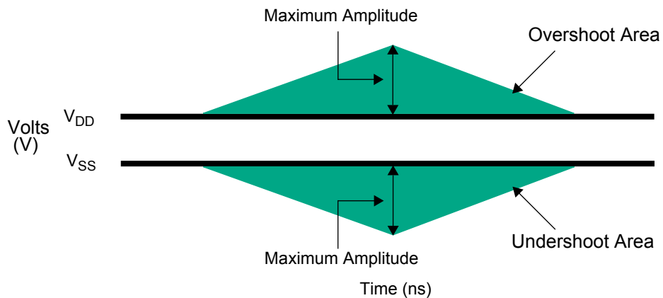
Figure 8. Address and Control Overshoot and Undershoot Definition
