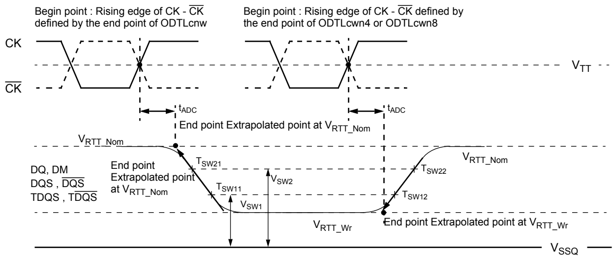
Figure 17. Definition of t_{\text{ADC}}
