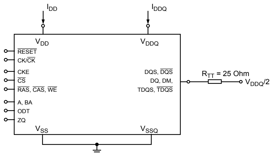
Figure 18. Measurement Setup and Test Load for IDD and IDDQ Measurements
