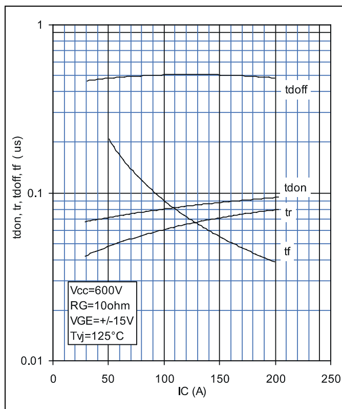
Fig. 7 Typ. Switching times vs on-state current
