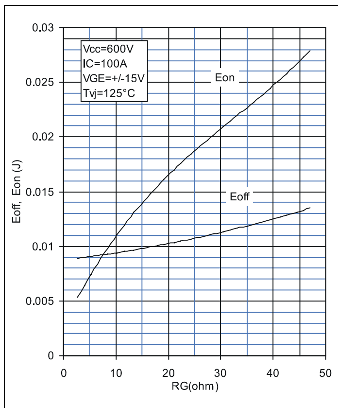
Fig. 6 Typ. Switching Energies per pulse vs gate resistor
