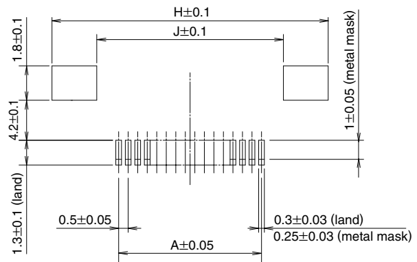
Space-saving type (FH28H)
