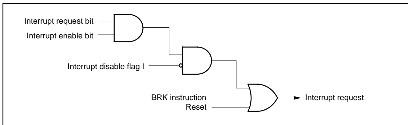
Fig. 13 Interrupt control
