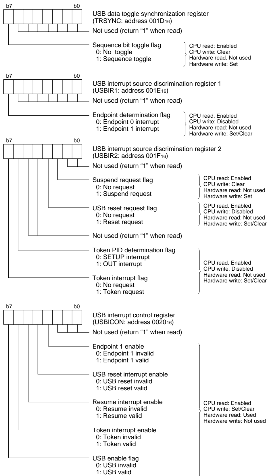
Fig. 25 Structure of serial I/O1-related registers (2)
