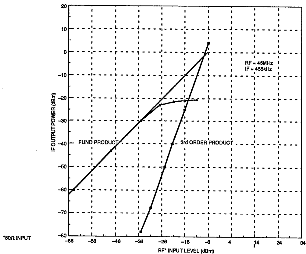
Figure 5. Mixer Third Order Intercept and Compression
