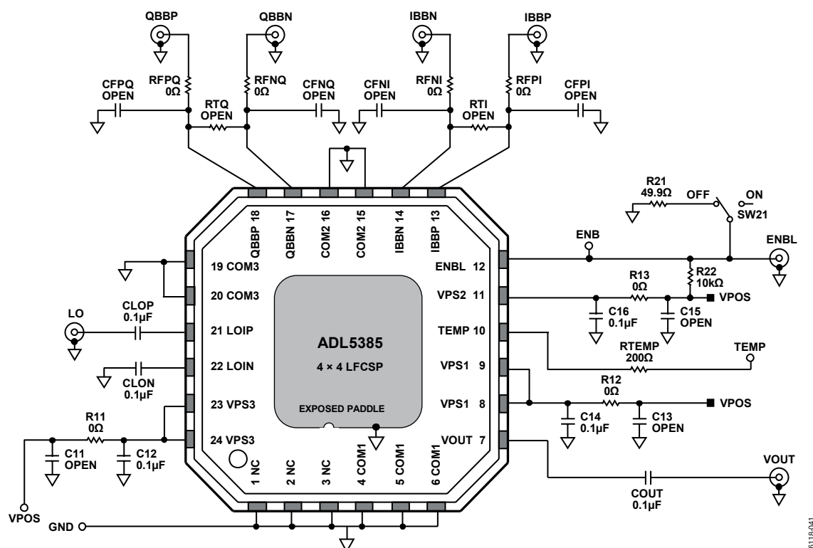
Figure 41. Evaluation Board Schematic
