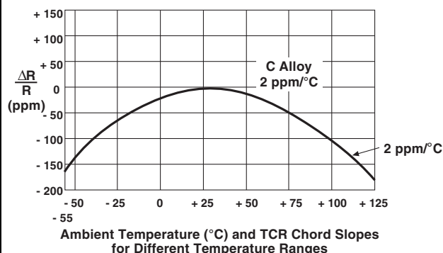
FIGURE 4 - TYPICAL RESISTANCE/TEMPERATURE CURVE
