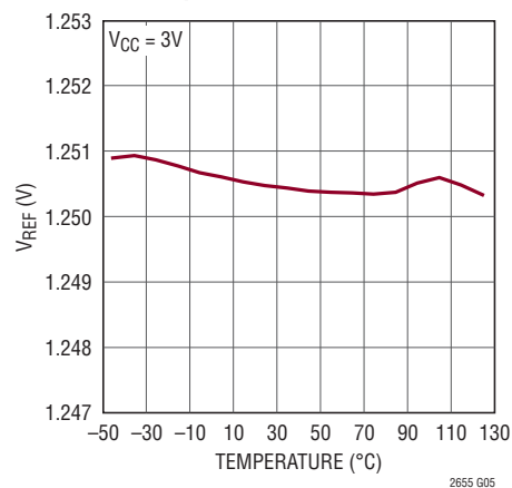
REFIN/OUT Output Voltage vs Temperature
