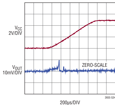
Power-On Reset Glitch
