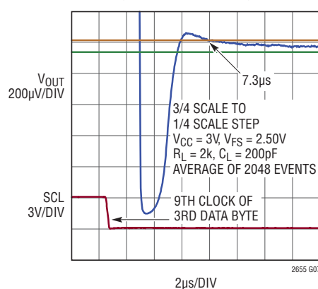
Settling to \pm 1\text{LSB} Falling
