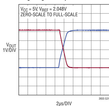
Large-Signal Response
