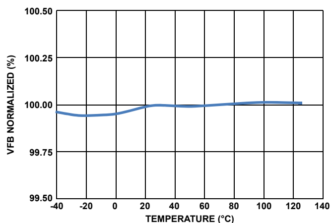
FIGURE 3. FEEDBACK ACCURACY
