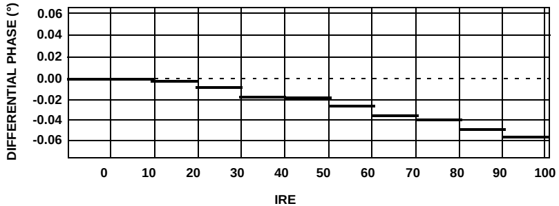
FIGURE 28. DIFFERENTIAL PHASE (°)
