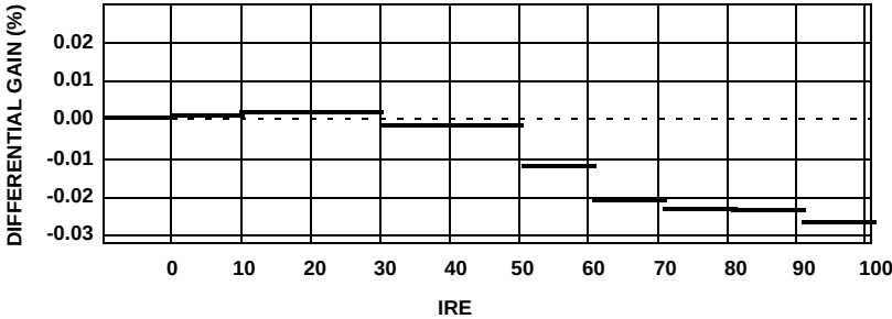
FIGURE 27. DIFFERENTIAL GAIN (%)
