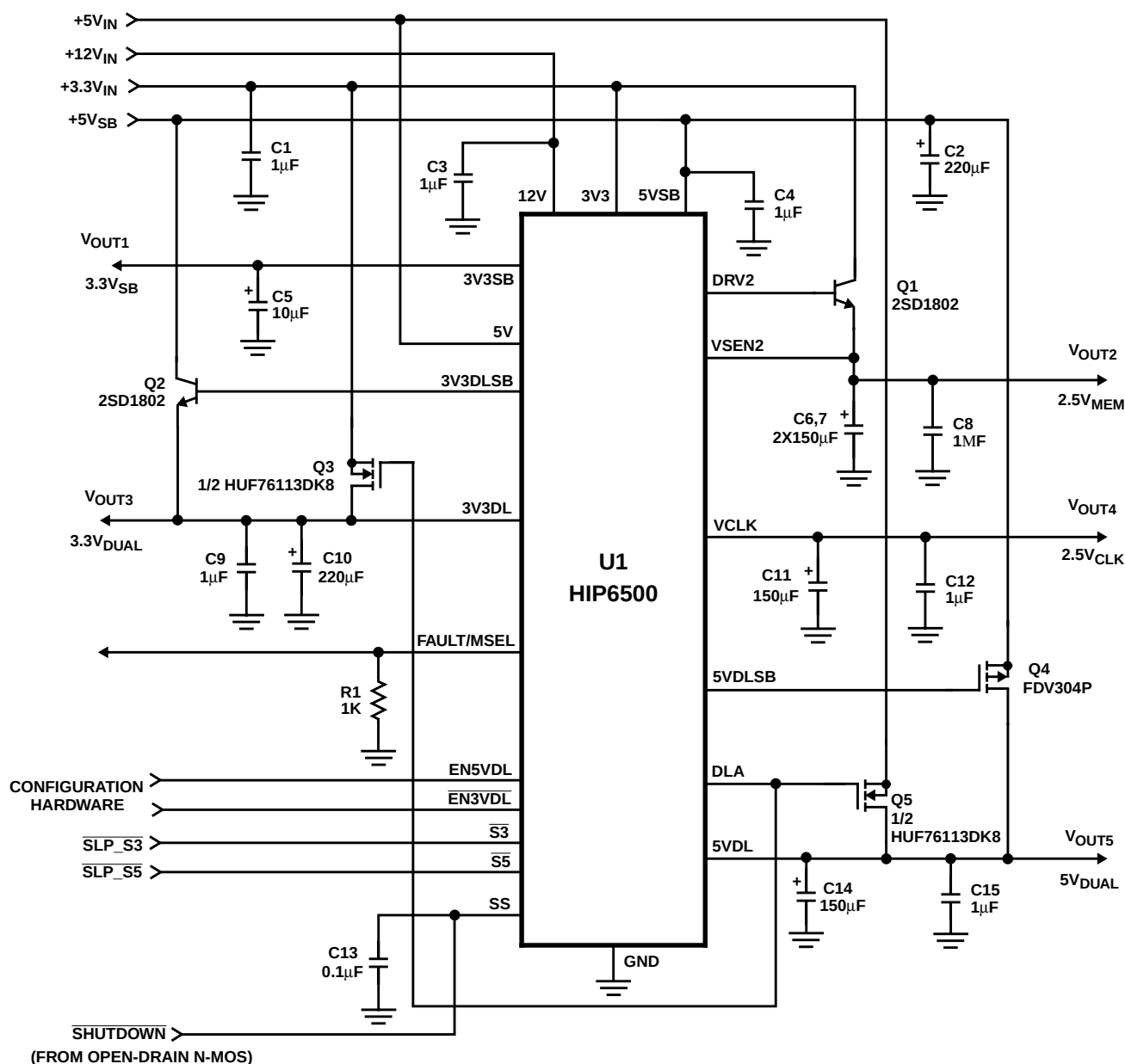
FIGURE 14. TYPICAL HIP6500 APPLICATION DIAGRAM
