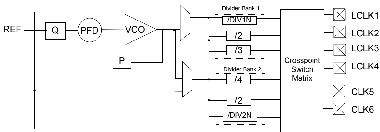
Figure 1. Basic PLL Block Diagram
