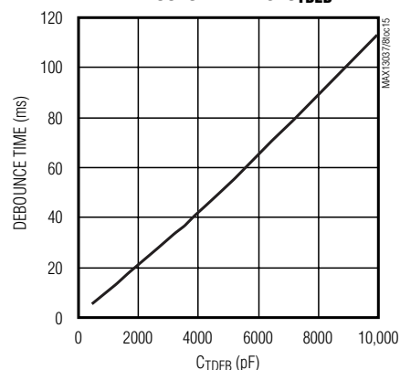
DEBOUNCE TIME vs. CTDEB
