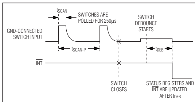
Figure 8. Switch Sampling in Scan Mode
