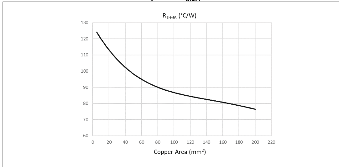
Figure 3. R_{thJA}
